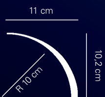
Art. 2077/Scomparsa Effetto a scomparsa sul soffitto Embossed effect on finished ceiling surface
